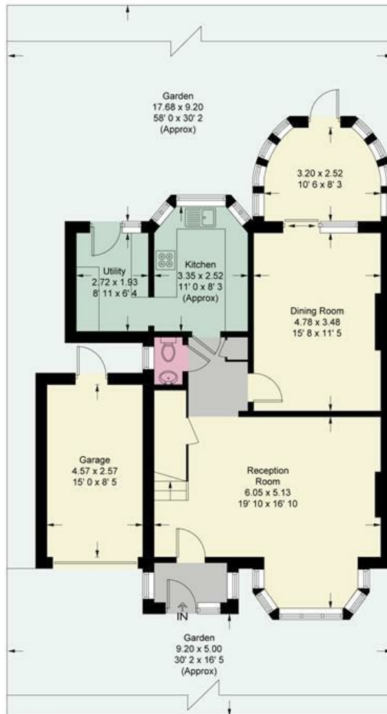
Ground Floor 846 sq ft / 78.6 sq m (Excluding Garage)
