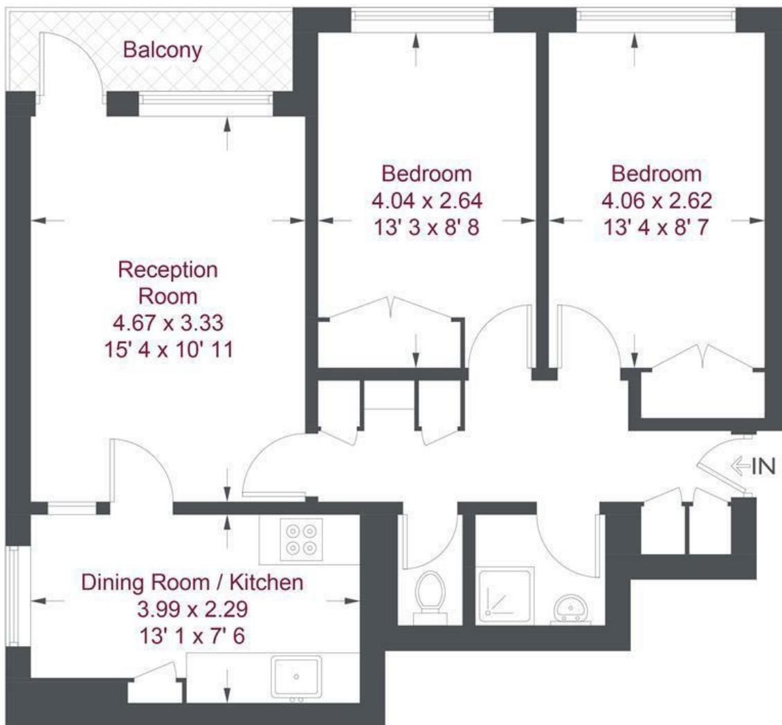
Eleventh Floor
