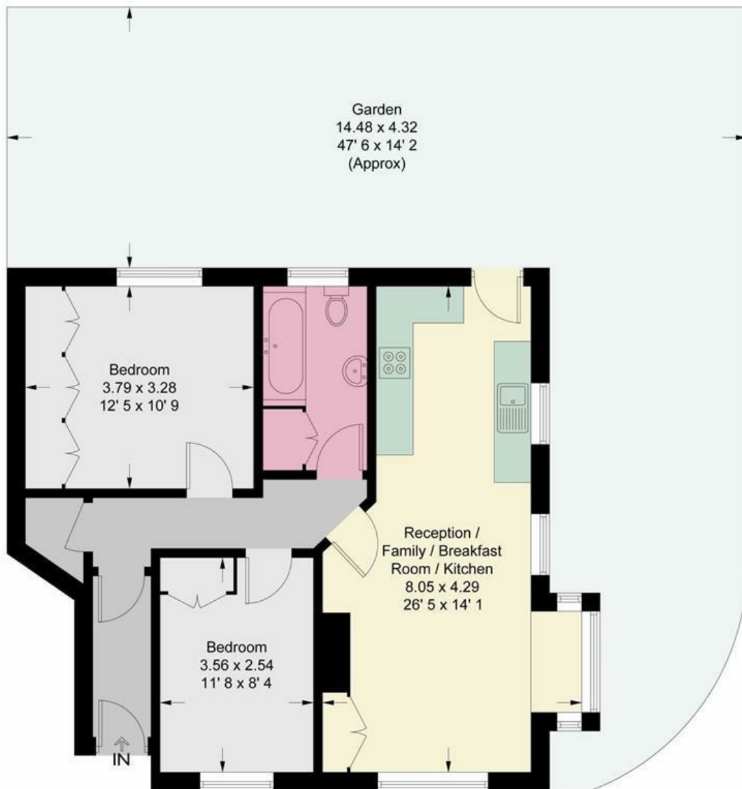
Ground Floor
