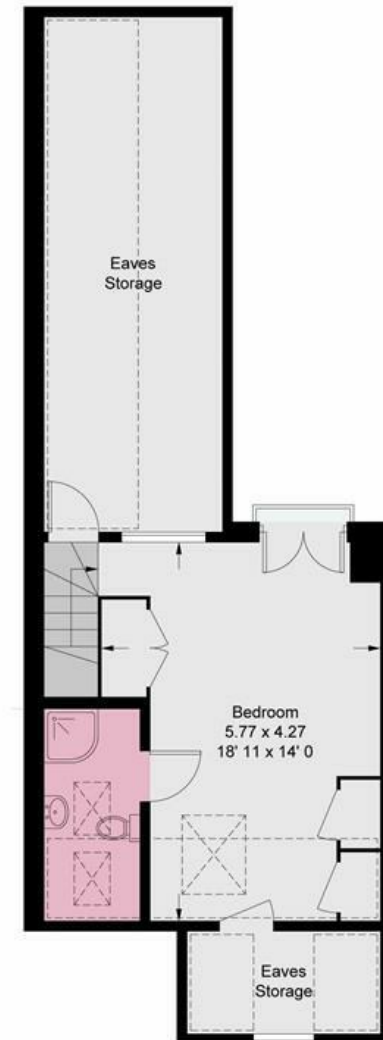
Second Floor 598 sq ft / 55.6 sq (Including Reduced Headroom / Eaves Storage)
