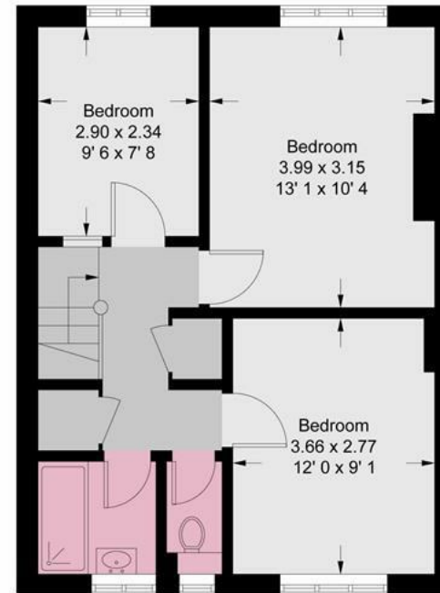
Third Floor 472 sq ft / 43.9 sq m
