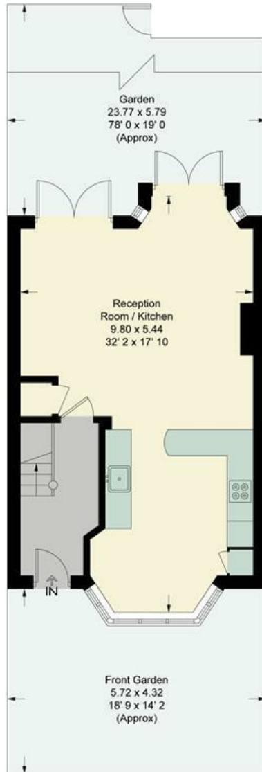
Ground Floor 518 sq ft / 48.1 sq m
