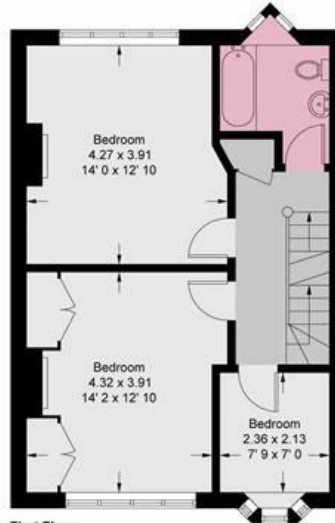
First Floor 553 sq ft / 51.4 sq m
