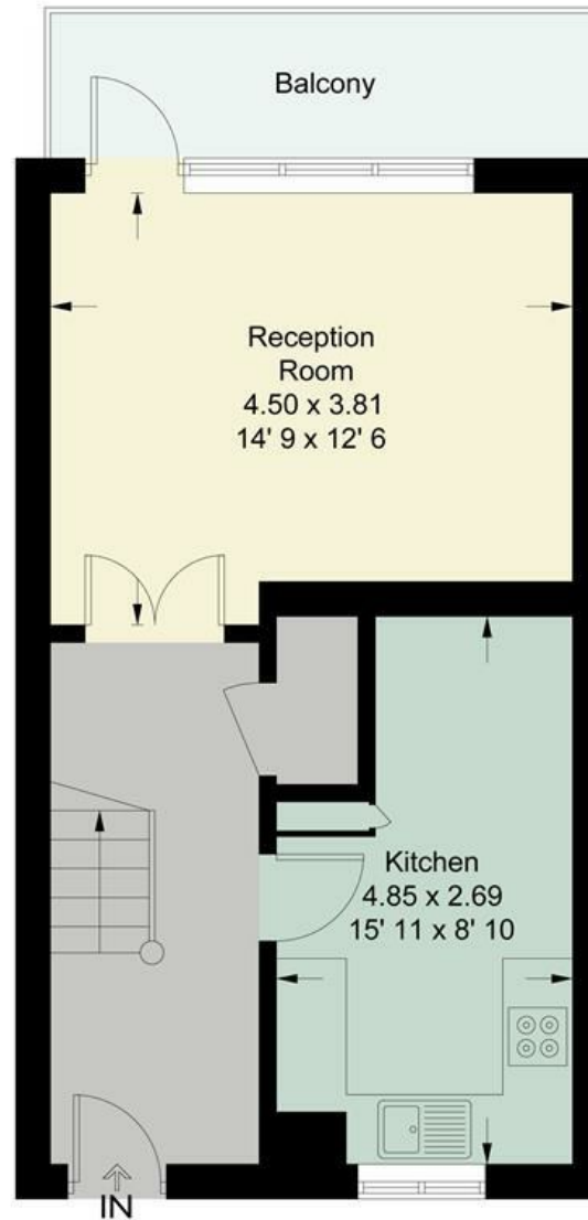
Third Floor 422 sq ft / 39.2 sq m
