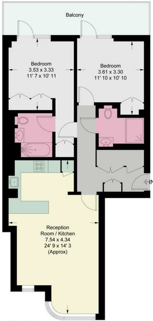
Third Floor
