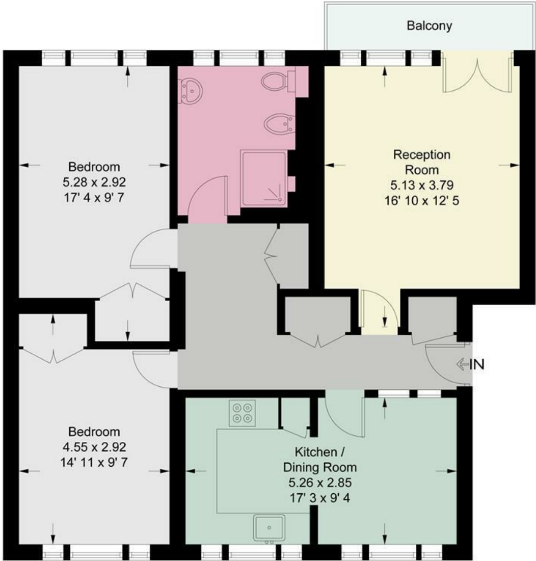
Third Floor
