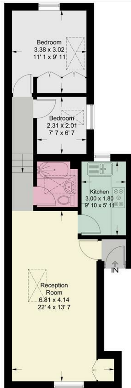
Second Floor
