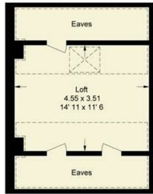
Second Floor 287 sq ft / 26.7 sq m (Including Reduced Headroom / Eaves)
