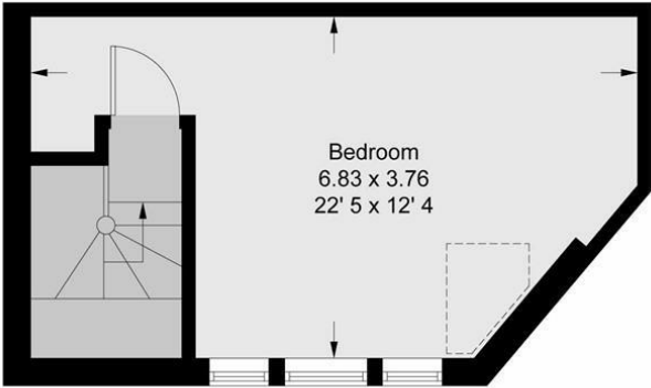
Third Floor 255 sq ft / 23.7 sq m (Including Reduced Headroom)
