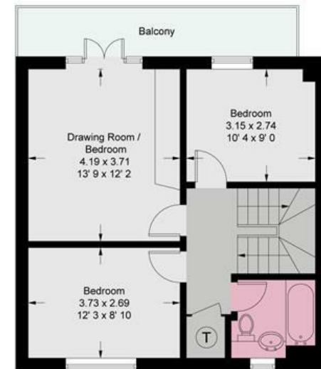
First Floor 534 sq ft / 49.6 sq m
