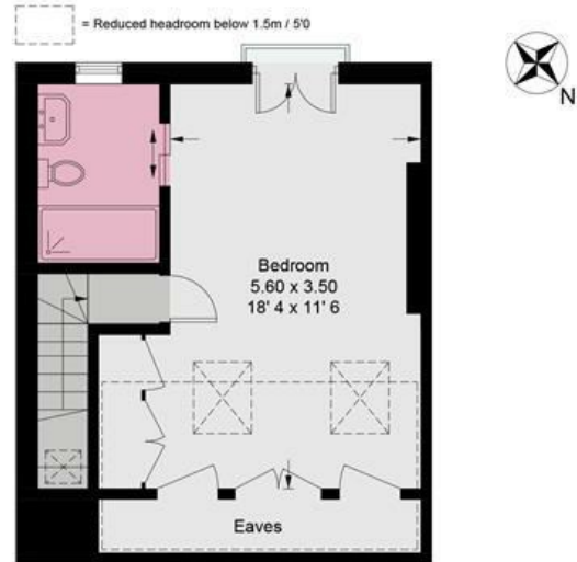
Second Floor 370 sq ft / 34.4 sq m (Including Reduced Headroom / Eaves)
