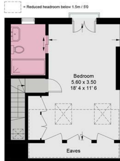
Second Floor 370 sq ft / 34.4 sq m (Including Reduced Headroom / Eaves)
