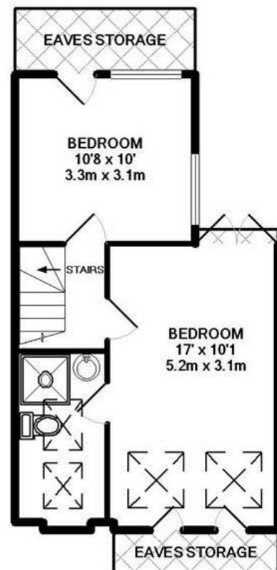
SECOND FLOOR APPROX. FLOOR AREA 34.2 SQ.M. (369 SQ.FT.)
