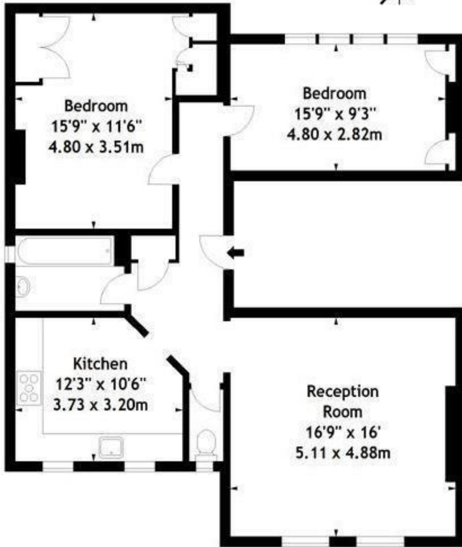
First Floor
